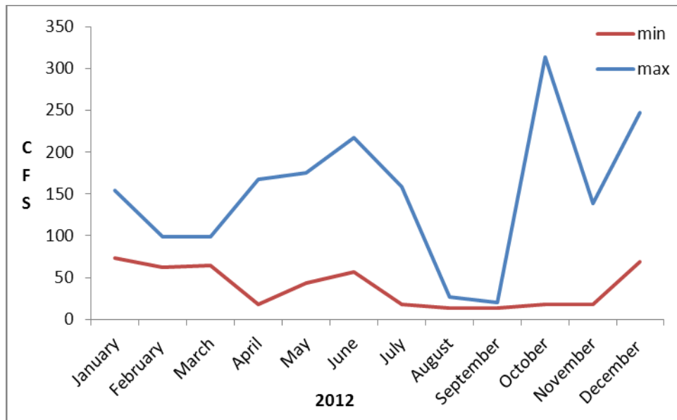
Figure 3. Tumalo Creek minimum and maximum monthly flows as recorded by the stream gauge located below Tumalo Irrigation District Canal. Data was missing before January 18 th , 2012. *This graph does not include water diverted from TIDC.
